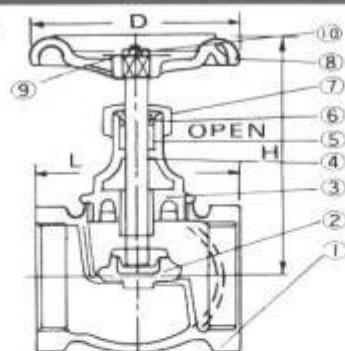
Fig. No. ST-301 Bronze disc, screwed bonnet, screwed ends.
